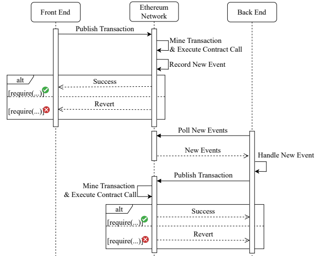
Figure 1: Typical workflow of Ethereum DApps.
